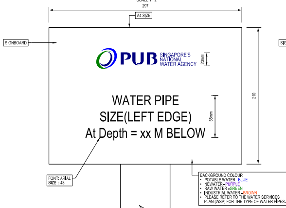
STANDARD DESIGN TO MARK OUT THE LEFT EDGE OF WATER PIPES ≥ 1200MM DIA.
