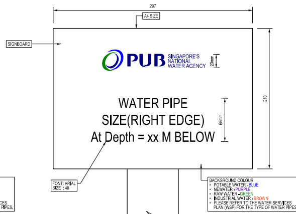
STANDARD DESIGN TO MARK OUT THE RIGHT EDGE OF WATER PIPES ≥ 1200MM DIA.
